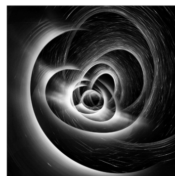
3 Particle Collider by Steve Peel
